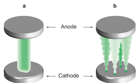
Fig. 26 : concentrated arcing [a] and diffused arcing [b].
