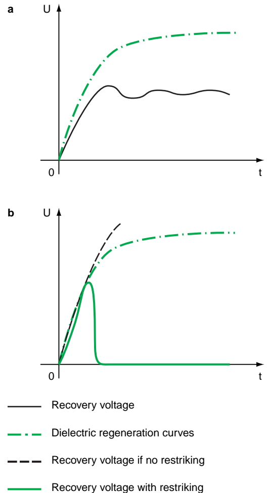
Fig. 6 : dielectric recovery curves: successful breaking [a] or dielectric failure [b].
