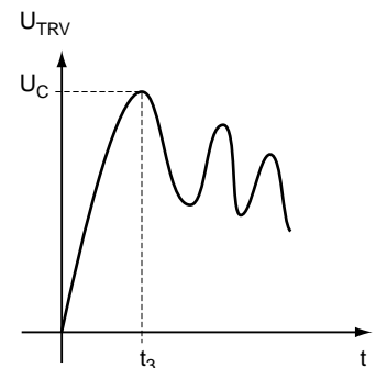
Fig. 7 : rated transient recovery voltage in the case of a short-circuit across the terminals of a circuit breaker (§ 4.102 IEC standard 60056).
