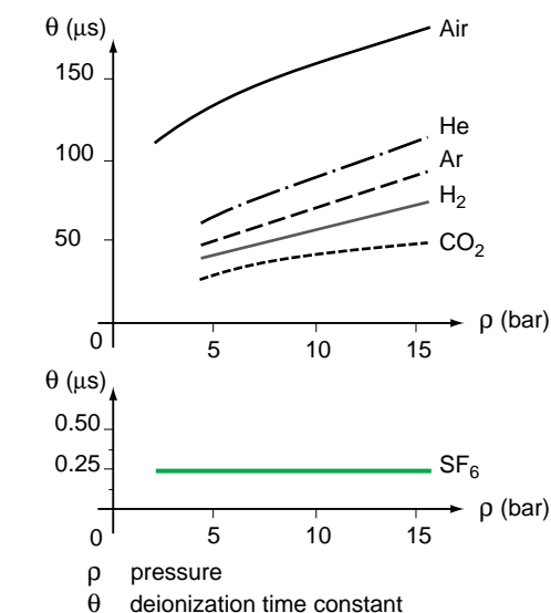
Fig. 19 : deionization time constants as a function of the pressure of various gases.
