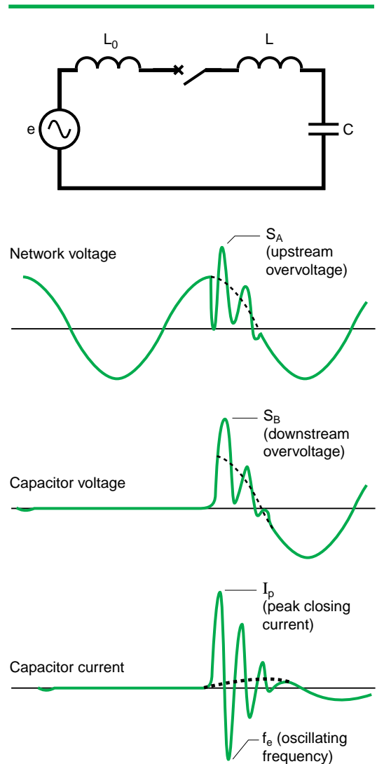
Fig. 13 : shapes of voltage and current (pre-strike overvoltage) during the coupling of a single stage capacitor to the network.
