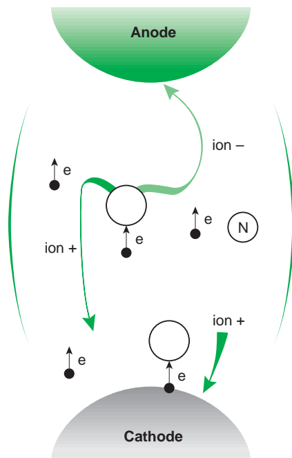
Fig. 4 : electrical arcing in a gaseous medium.
